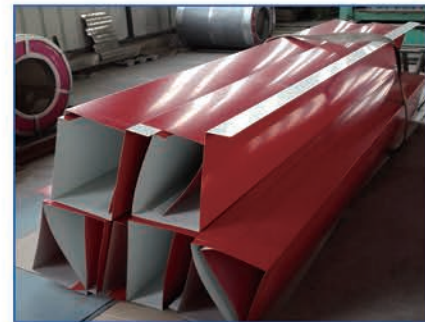
waterproof eaves 防水檐
